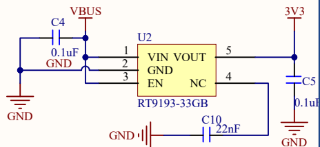
RT9193-33GB
